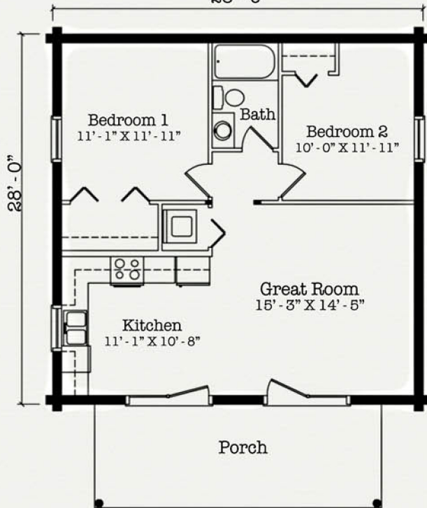
Floor Plan "B"
