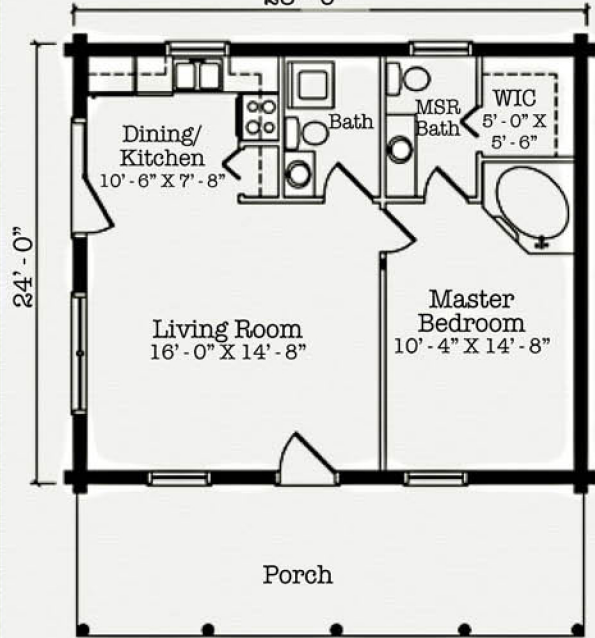
Floor Plan "A"
