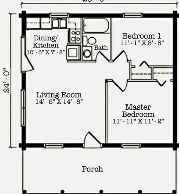
Floor Plan "B"
