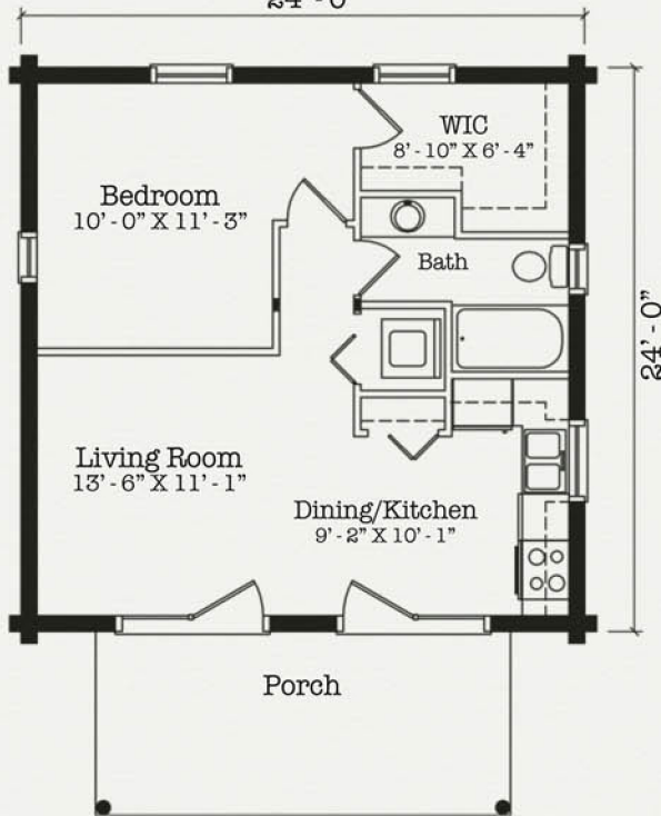
Floor Plan "A"
